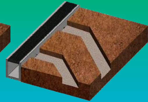
Step3. Laying gravel
